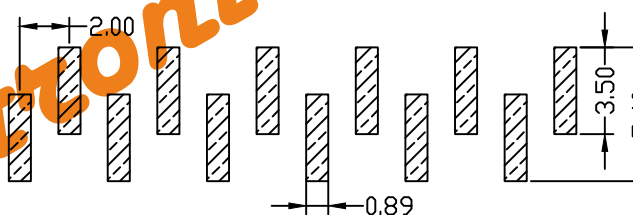
TYPE B PCB LAYOUT
